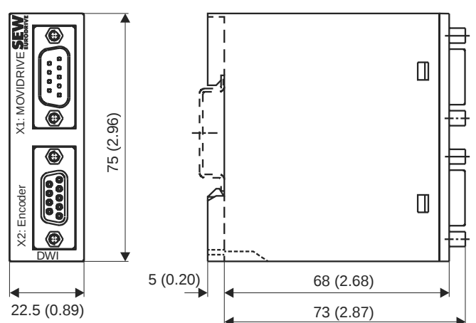
Figure 28: Dimensions, DWI11A, in mm (in)
