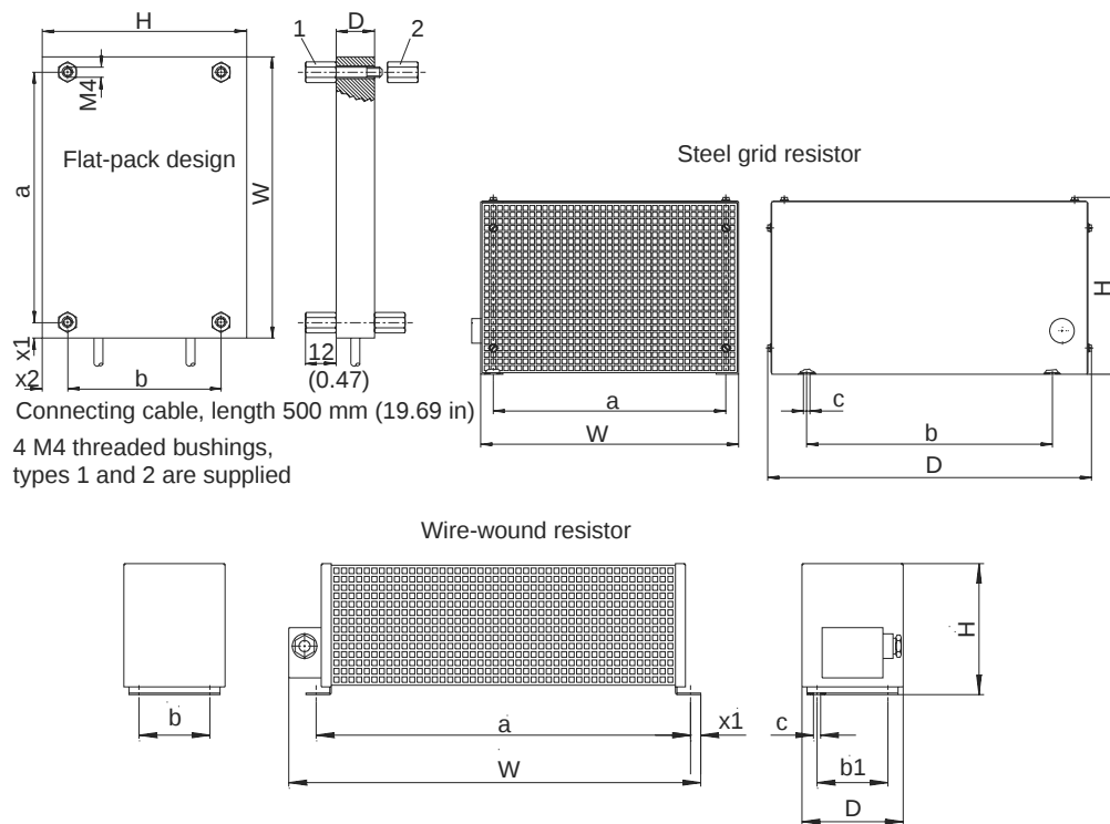
Figure 32: Dimensions, BW... braking resistors
