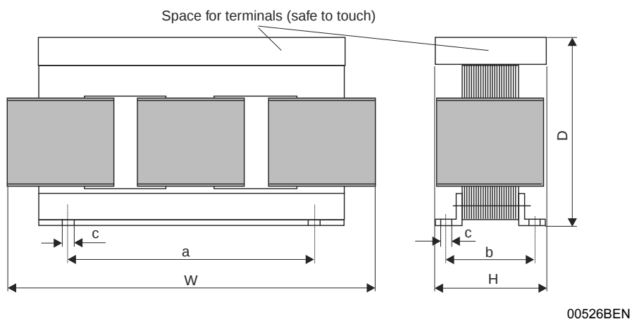
Figure 33: Dimensions, ND... line chokes
