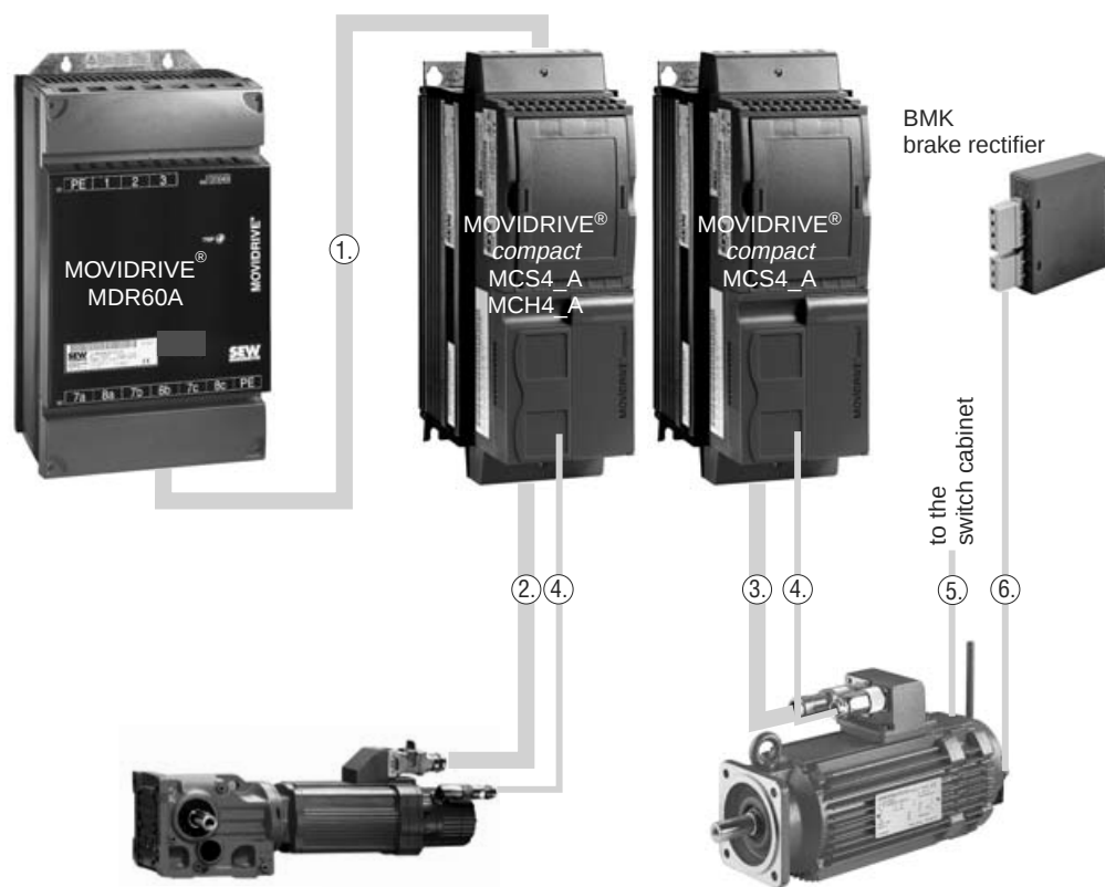
Figure 39: Cable sets for the MOVIDRIVE® compact system
