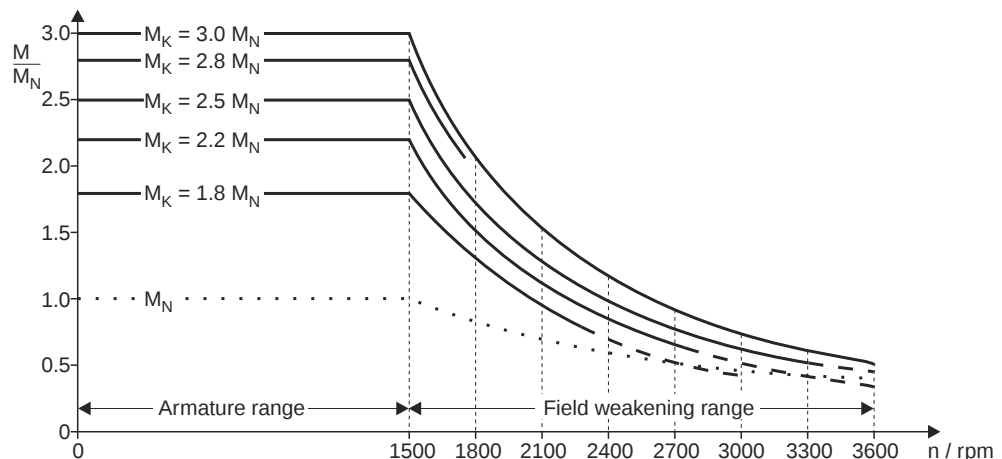
Figure 43: Quadratically falling breakdown torque
