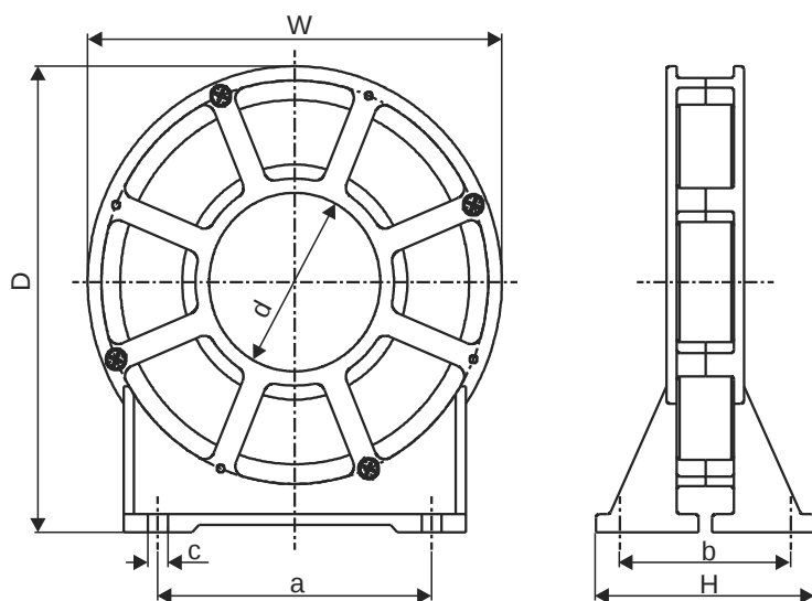
Figure 35: Dimensions, HD... output chokes
