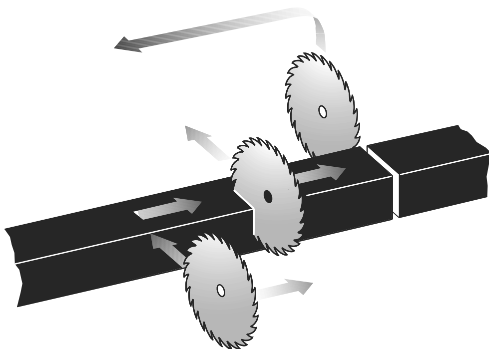
Figure 5: Typical application for the 'internal synchronous operation'
