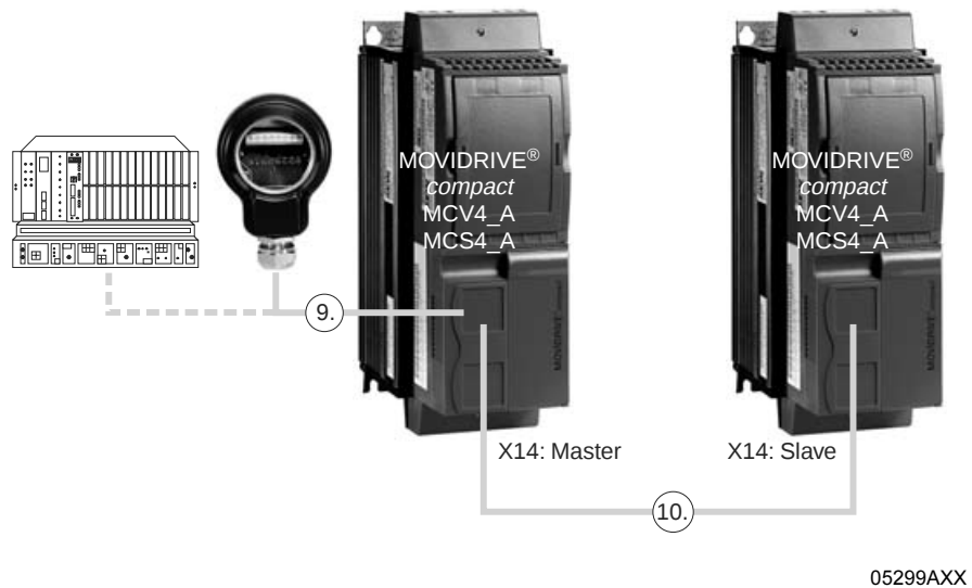
Figure 41: Connection of external encoder and master/slave connection
